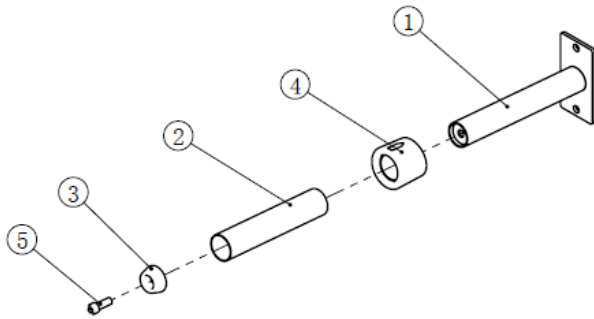
16. Lat Bar Assy
