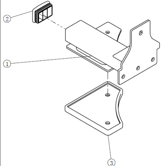
15. Short Weight Plate Storage Assy
