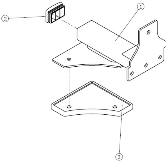
9.1 Left Safety Rail First Assy
