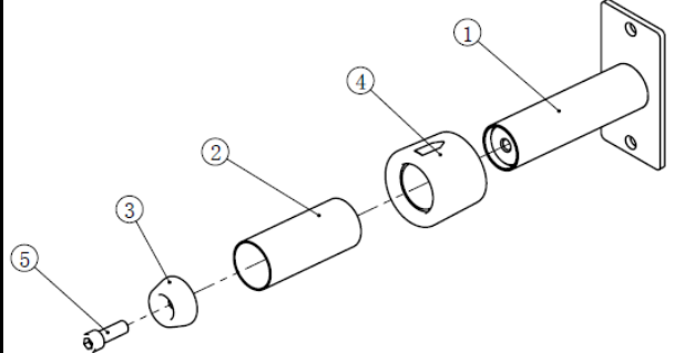
15. Short Weight Plate Storage Assy
