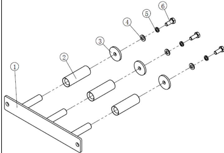
17. Rubber Band Rack Assy
