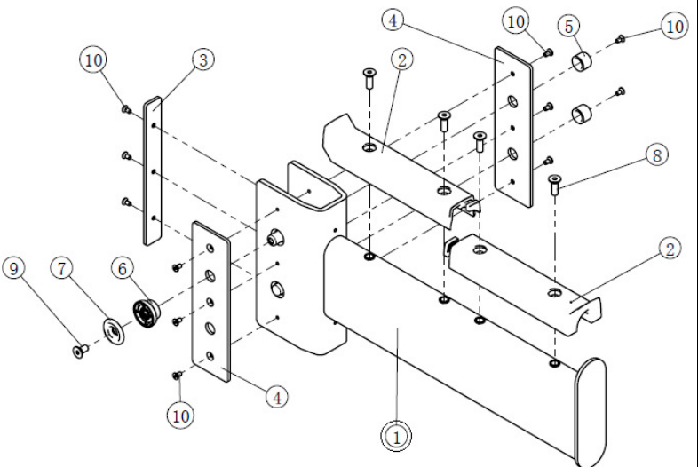
11. Left Weight Hook Assy
