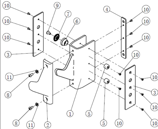
14. Long Weight Plate Storage Assy
