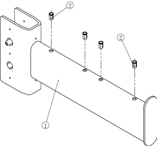
10.1 Right Safety Rail First Assy
