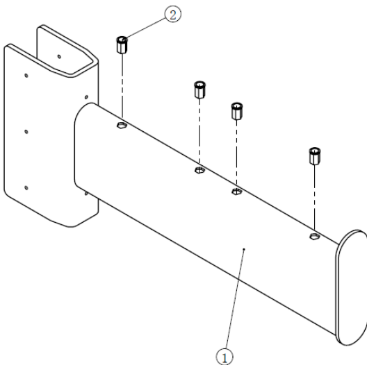
10.1 Right Safety Rail First Assy
