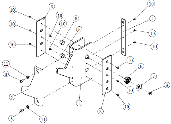
11. Left Weight Hook Assy
